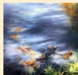
SUNSPOTS
